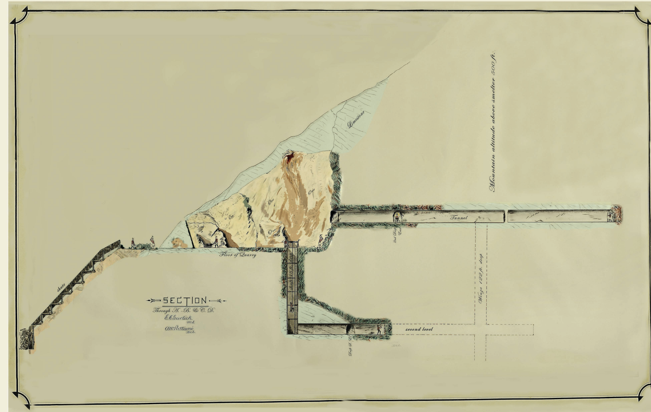
1881 CROSS-SECTION OF LINES A - B ON THE FIRST LEVEL AND C - D OF THE SECOND LEVEL OF THE COPPER QUEEN MINE
